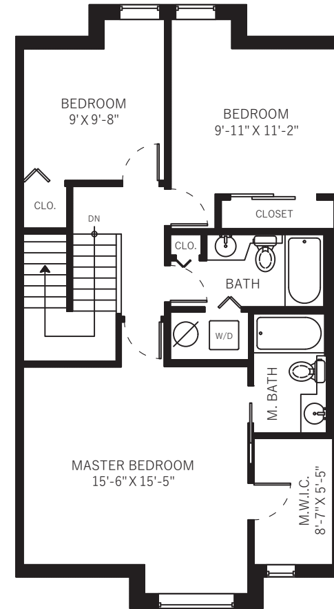
Upper Floor: 864 Sq.Ft. Ceiling Height: 8' / Max: 10'
